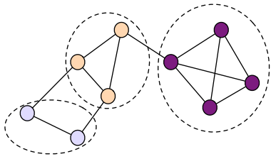
Figure 2: A clique cover of a graph of accesses. Nodes represent accesses while edges represent at least a threshold level of similarity between edges.
