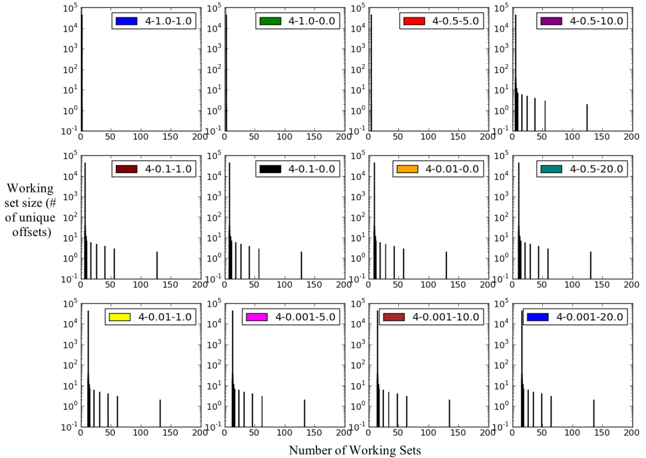
Figure 8: The Bag-of-Edges technique with varying offset and time scaling. Each graph is labeled as number of levels - offset scaling factor - time scaling factor.
