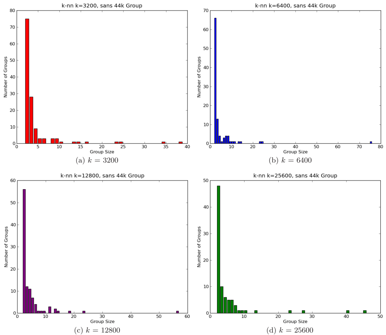
Figure 6: Working sets with k -Nearest Neighbor. If k is very high or low, fewer large groups are found.
