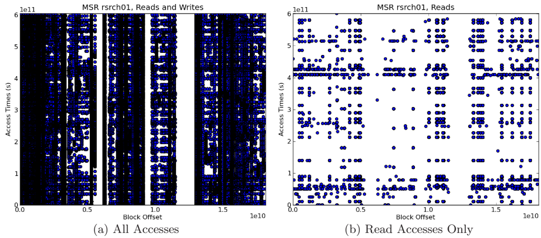
Figure 3: Block access over time for all accesses and only reads
