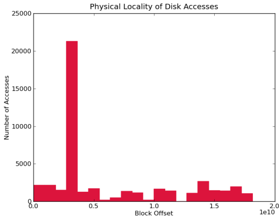
Figure 4: Visualizing the locality as a histogram exposes a localized spike in accesses.
