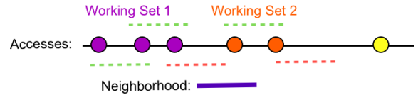
Figure 1: Neighborhood partitioning
