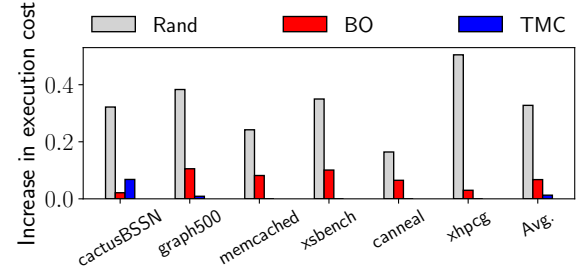
Figure 6: Execution cost increase over exhaustive search
