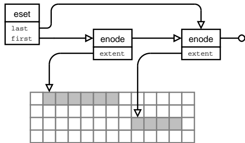
Figure 5: LiFS extent system for disk allocation
