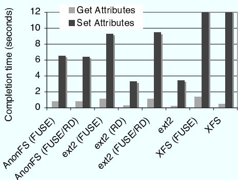
(b) Setting and getting file attributes on 15,620 files ( k = 5 , d = 5 , n = 4 , a = 20 ). The times are in seconds and averaged over 5 runs. RD indicates file system on RAM-disk. Again, XFS, both with and without FUSE, was much slower, requiring over 109 seconds to complete the set attributes benchmark. The graph was cut off to show detail for the other file systems.
